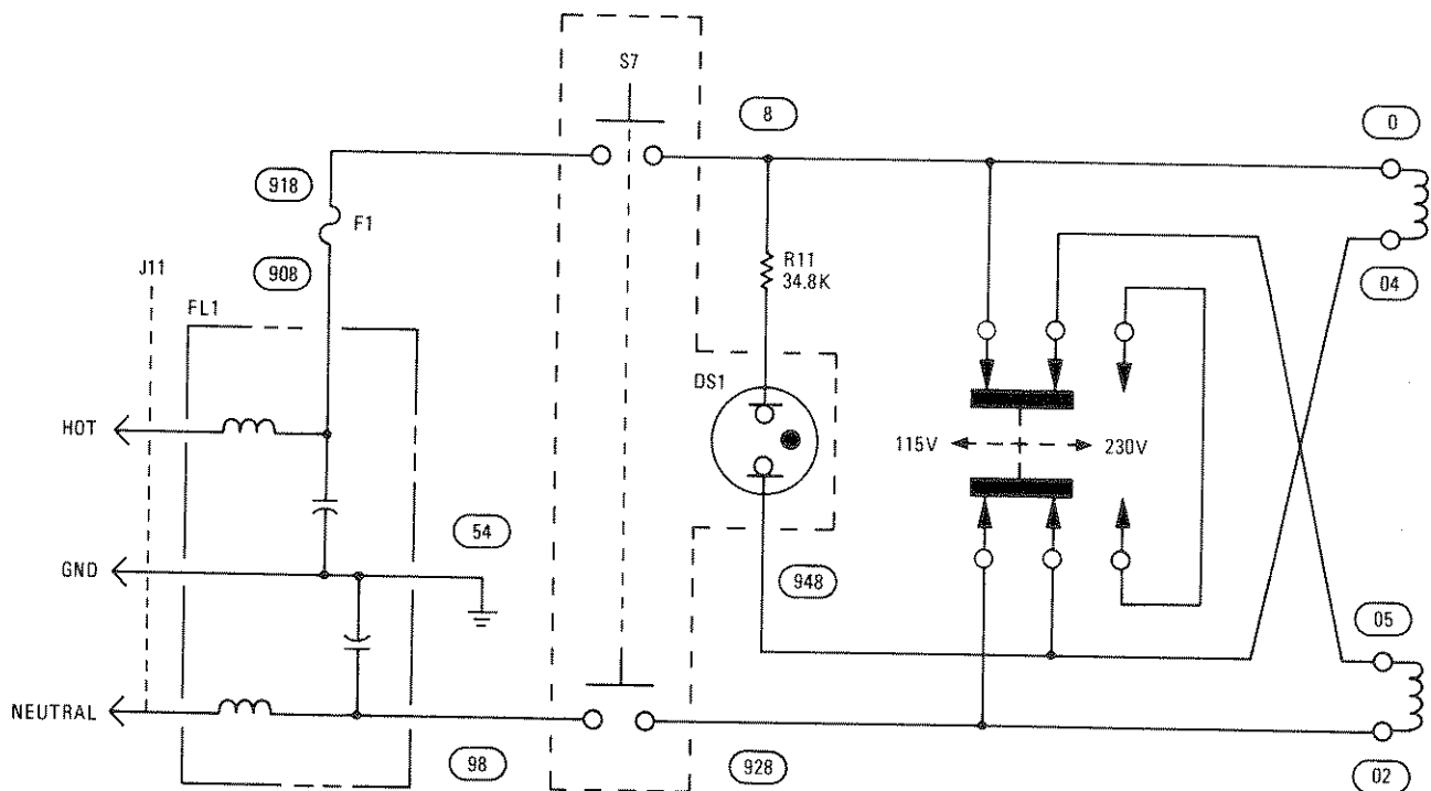
Figure 7-19. Primary Wiring Change (Change 29)
